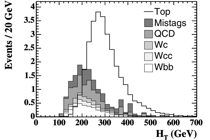
FIG. 15. Distribution of the H_T variable for t\bar{t} Monte Carlo, and for various backgrounds normalized to an integrated luminosity of 107 \text{ pb}^{-1} .
