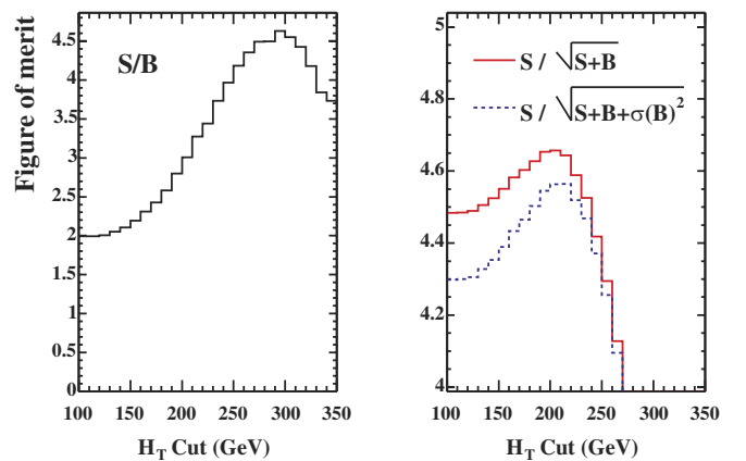
FIG. 16 (color online). Estimate of S/B , statistical and total significance for 107 \text{ pb}^{-1} integrated luminosity, as a function of H_T cut.
